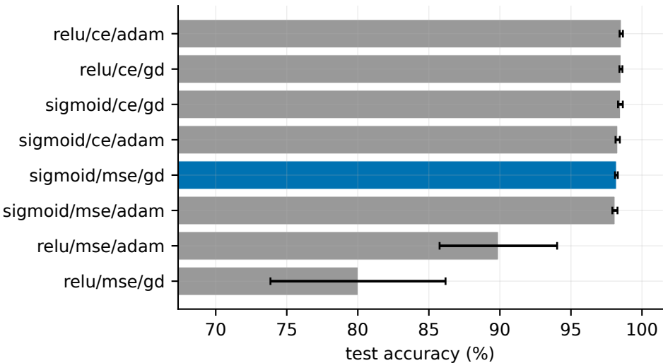
Configuration ablation — Optdigits (10 classes)
