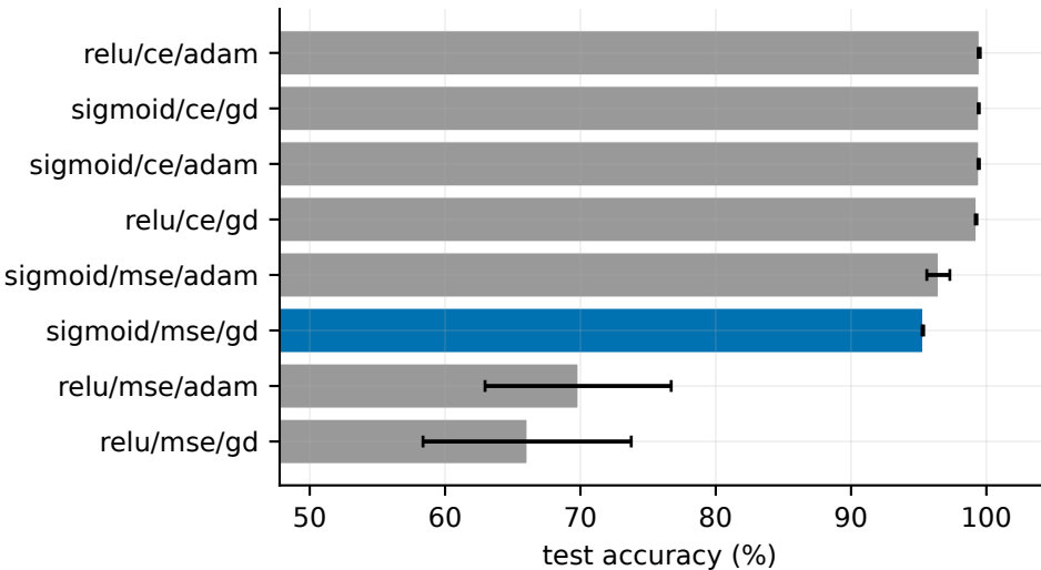
Configuration ablation — Pendigits (10 classes)
