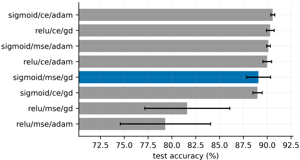
Configuration ablation — Satimage (6 classes)
