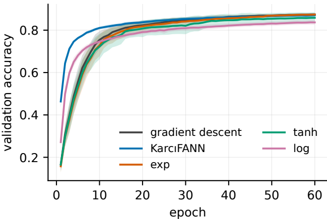
Convergence — Letter (26 classes) (mean \pm 1 SD over 16 seeds)
