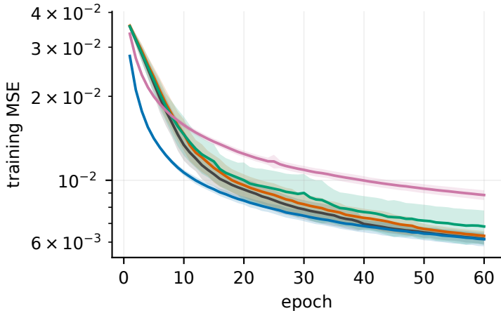
Convergence — Letter (26 classes) (mean \pm 1 SD over 16 seeds)
