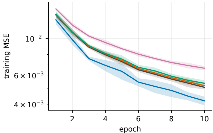
Convergence — MNIST (10 classes) (mean \pm 1 SD over 16 seeds)
