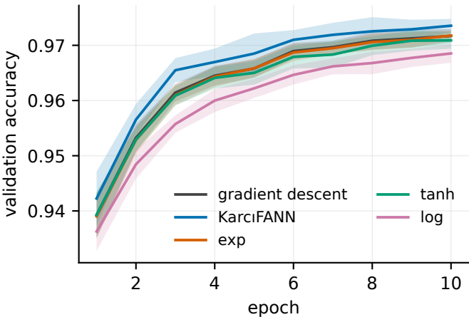
Convergence — MNIST (10 classes) (mean \pm 1 SD over 16 seeds)
