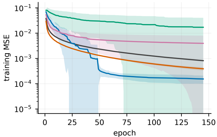
Convergence — Optdigits (10 classes) (mean \pm 1 SD over 16 seeds)
