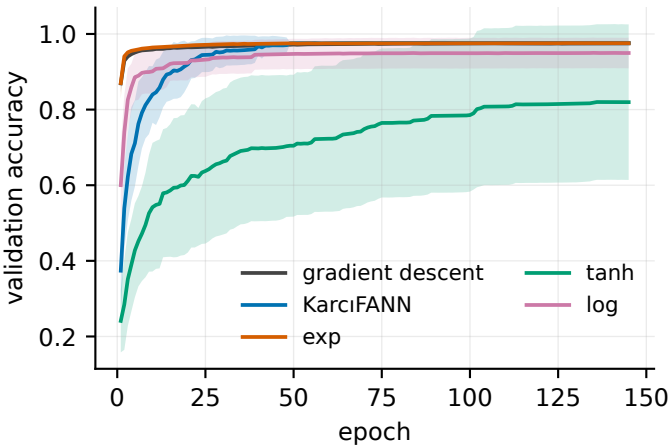
Convergence — Optdigits (10 classes) (mean \pm 1 SD over 16 seeds)
