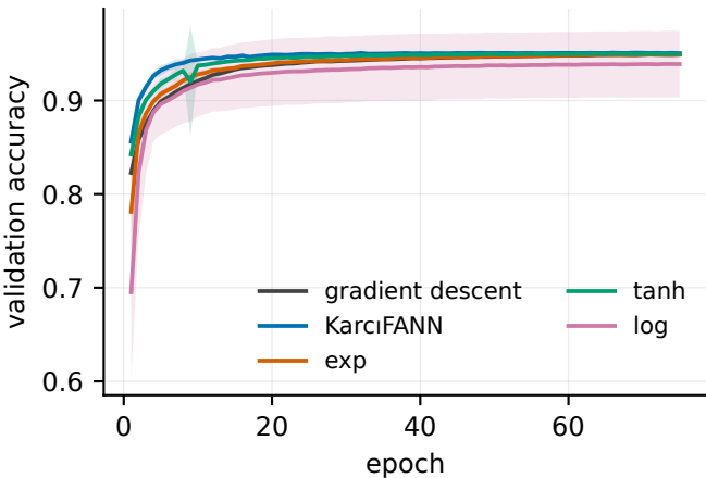
Convergence — Pendigits (10 classes) (mean \pm 1 SD over 16 seeds)
