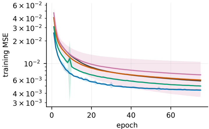
Convergence — Pendigits (10 classes) (mean \pm 1 SD over 16 seeds)
