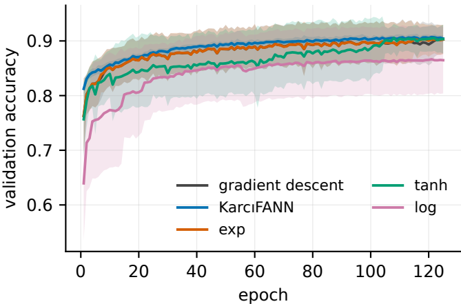
Convergence — Satimage (6 classes) (mean \pm 1 SD over 16 seeds)
