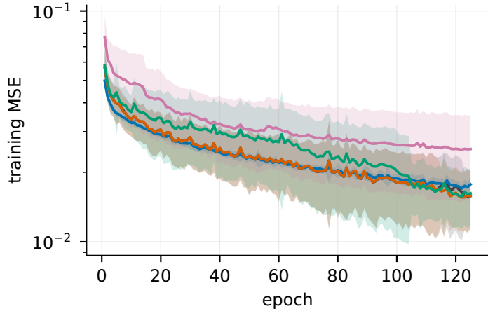
Convergence — Satimage (6 classes) (mean \pm 1 SD over 16 seeds)
