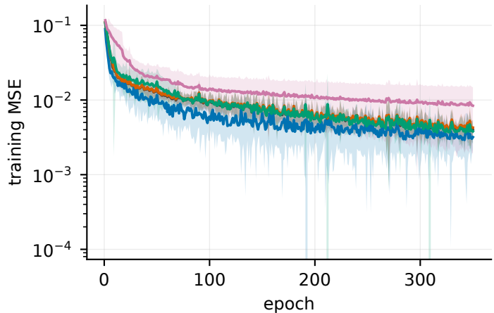
Convergence — Segment (7 classes) (mean \pm 1 SD over 16 seeds)
