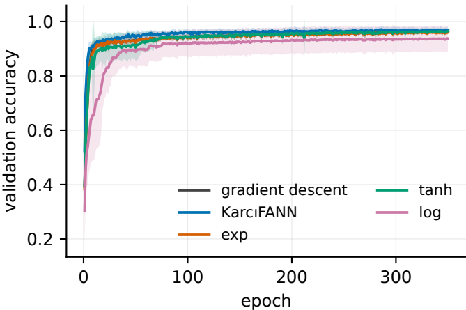
Convergence — Segment (7 classes) (mean \pm 1 SD over 16 seeds)
