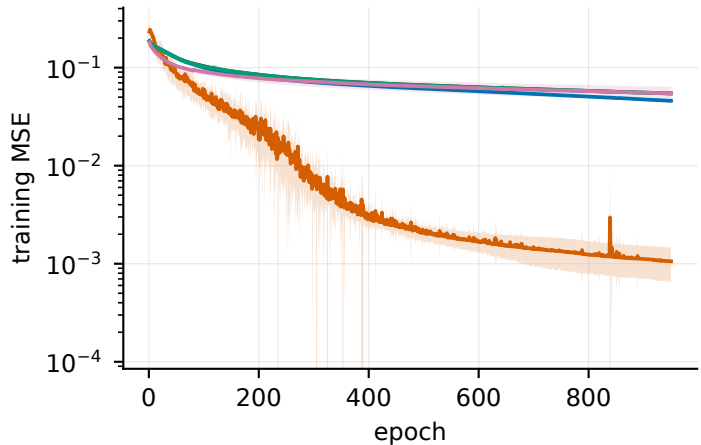
Convergence — Vehicle (4 classes) (mean \pm 1 SD over 16 seeds)
