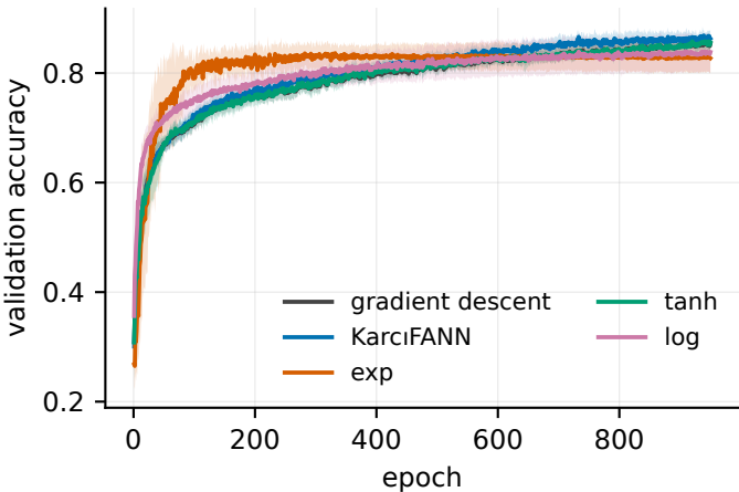
Convergence — Vehicle (4 classes) (mean \pm 1 SD over 16 seeds)
