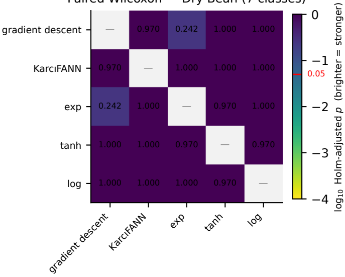
Paired Wilcoxon — Dry Bean (7 classes)
