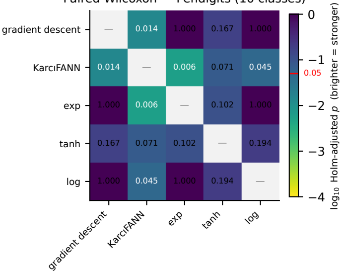
Paired Wilcoxon — Pendigits (10 classes)
