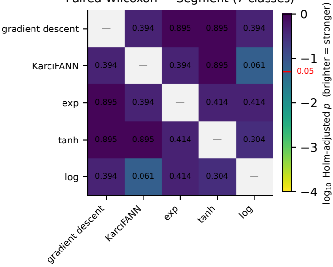
Paired Wilcoxon — Segment (7 classes)
