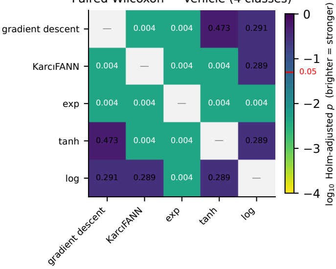
Paired Wilcoxon — Vehicle (4 classes)
