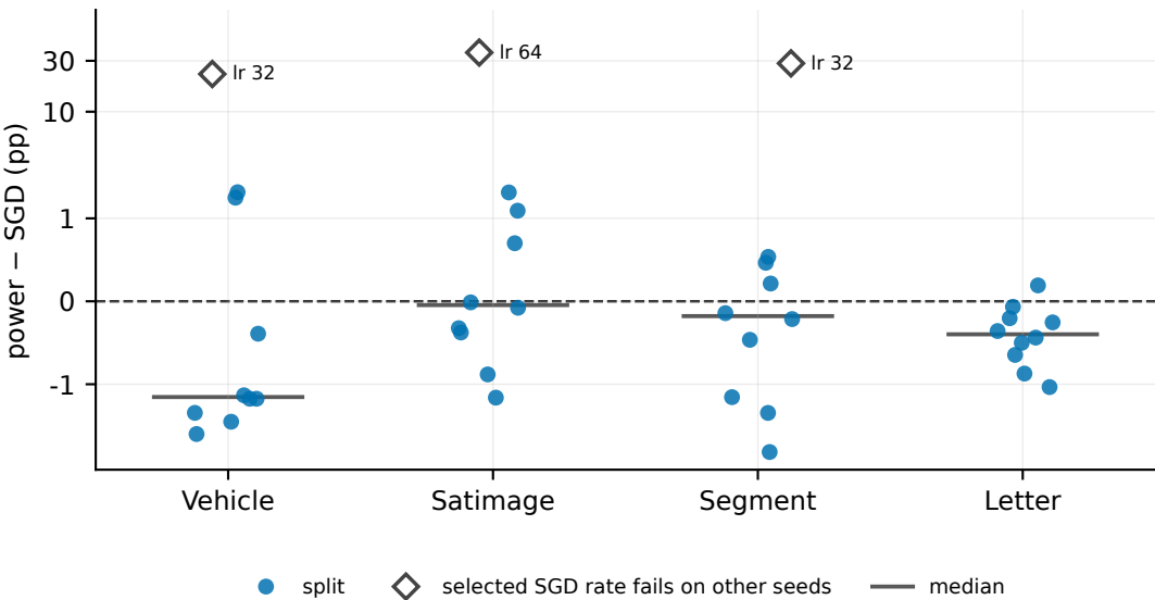
Per-split differences, tuning nested inside each split
