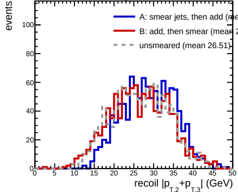
Jet20, R=0.2 , 40 < p_T^{\text{lead}} < 50 GeV, jets selected
