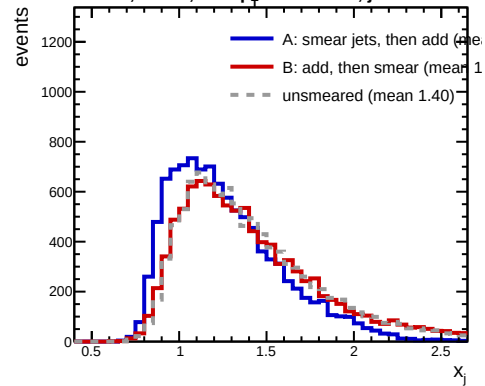
Jet20, R=0.3 , 30 < p_T^{\text{lead}} < 35 GeV, jets selected
