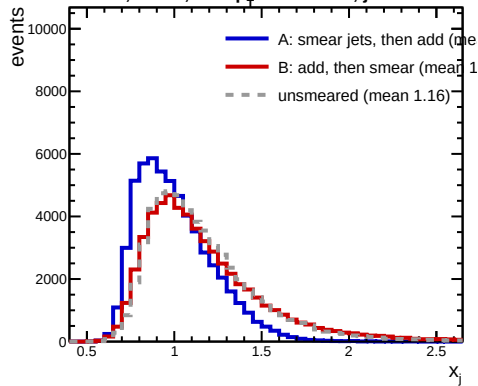
Jet20, R=0.3 , 20 < p_T^{\text{lead}} < 25 GeV, jets selected
