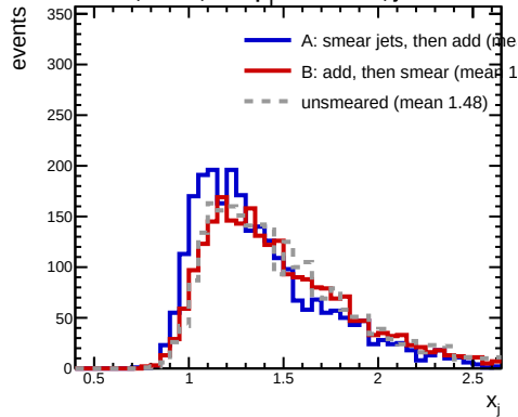
Jet20, R=0.3 , 35 < p_T^{\text{lead}} < 40 GeV, jets selected
