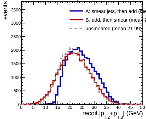
Jet20, R=0.2 , 25 < p_T^{\text{lead}} < 30 GeV, jets selected
