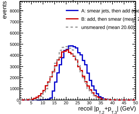
Jet20, R=0.2 , 20 < p_T^{\text{lead}} < 25 GeV, jets selected
