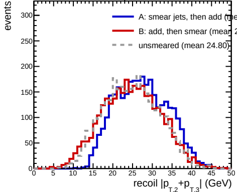
Jet20, R=0.2 , 35 < p_T^{\text{lead}} < 40 GeV, jets selected
