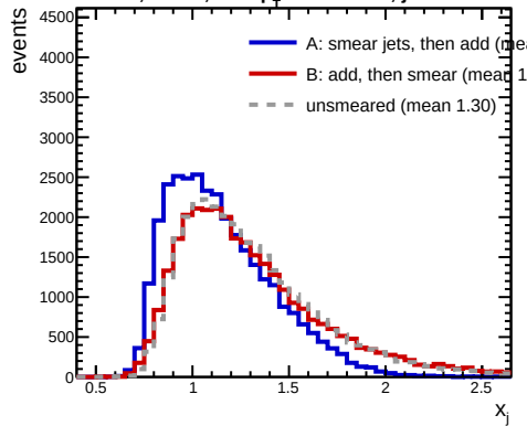
Jet20, R=0.3 , 25 < p_T^{\text{lead}} < 30 GeV, jets selected
