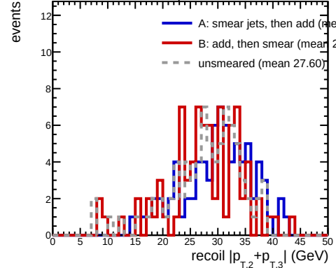
Jet20, R=0.2 , 50 < p_T^{\text{lead}} < 60 GeV, jets selected
