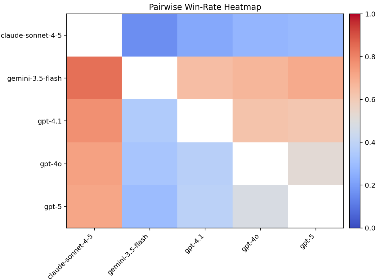
Figure 13: Pairwise model win-rate heatmap across benchmarks.
