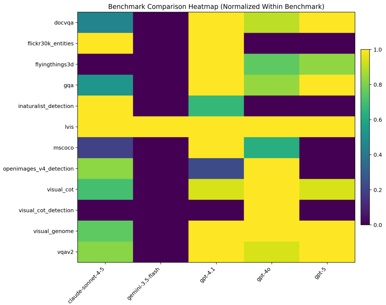
Figure 7: Normalized score heatmap across models and benchmarks.
