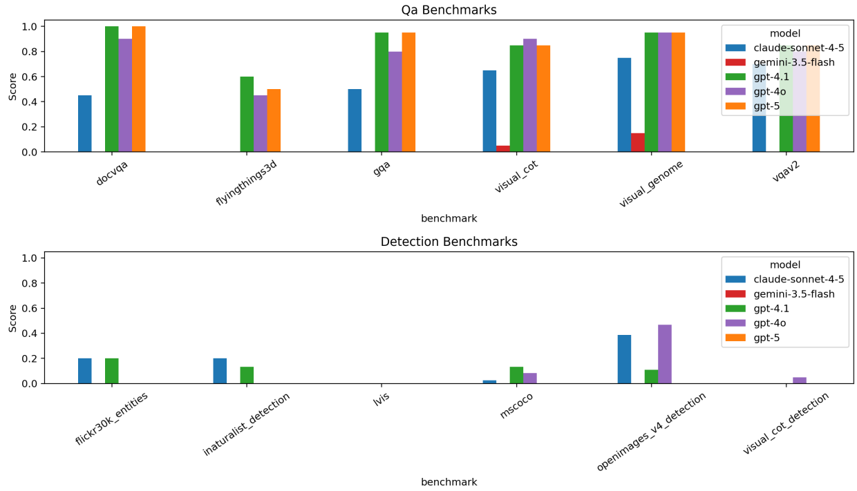
Figure 13: Small multiples for Type A and Type B benchmark families.
