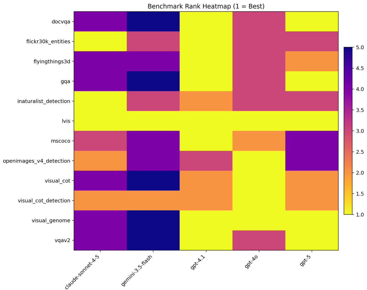
Figure 8: Rank heatmap across models and benchmarks.
