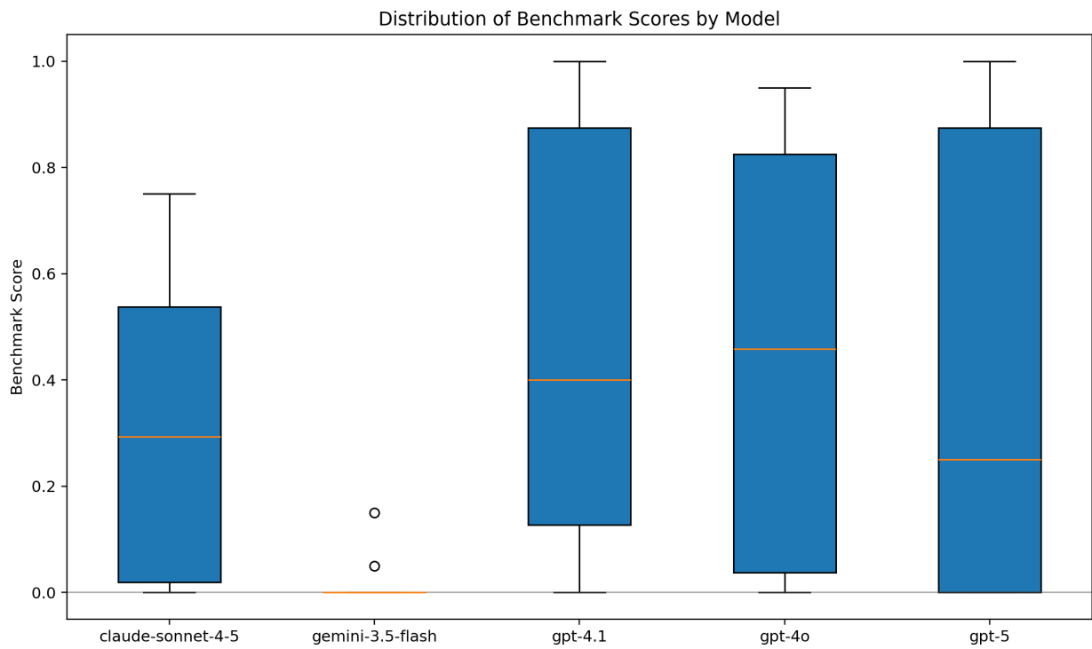
Figure 4: Distribution of benchmark scores by model.
