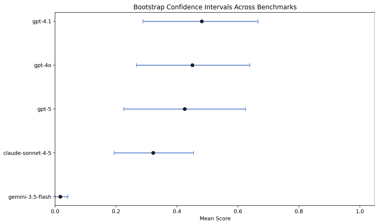
Figure 5: Bootstrap confidence intervals for mean benchmark score.
