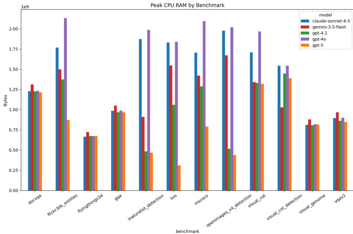
Figure 18: Peak CPU RAM by benchmark.
