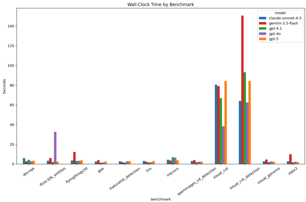
Figure 17: Wall-clock time by benchmark.
