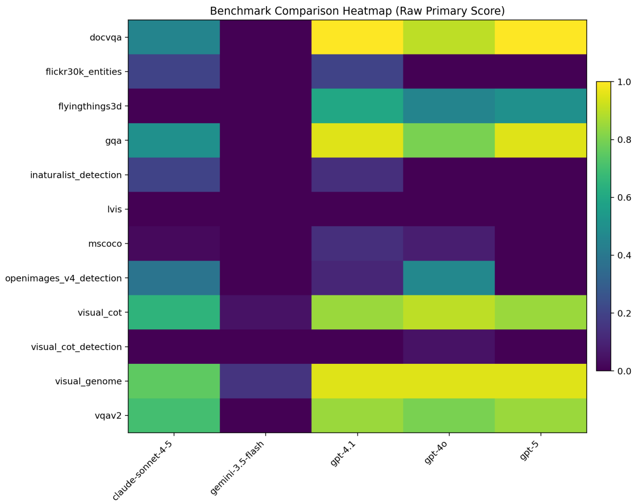
Figure 6: Raw score heatmap across models and benchmarks.
