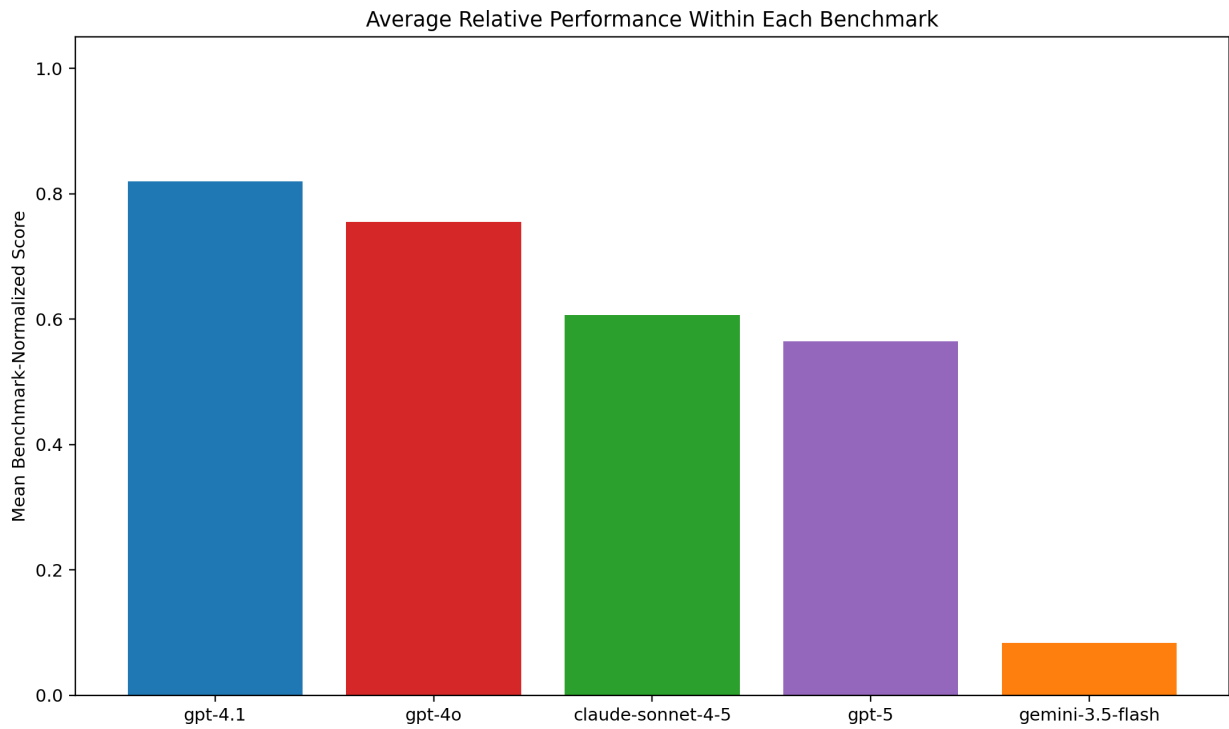
Figure 2: Mean normalized score for the five API models.
