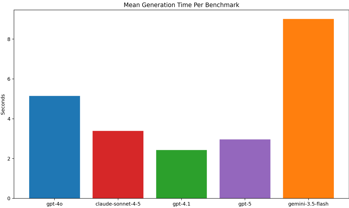
Figure 15: Mean generation time by model.
