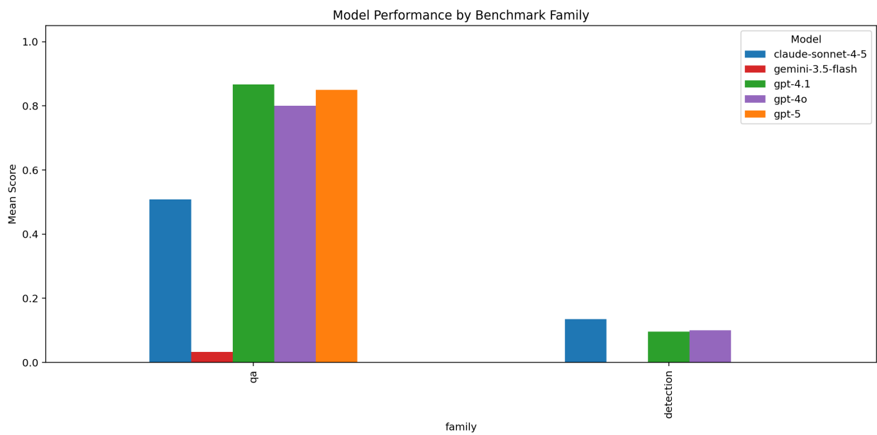
Figure 11: Grouped bar chart for Type A QA and Type B detection benchmarks.
