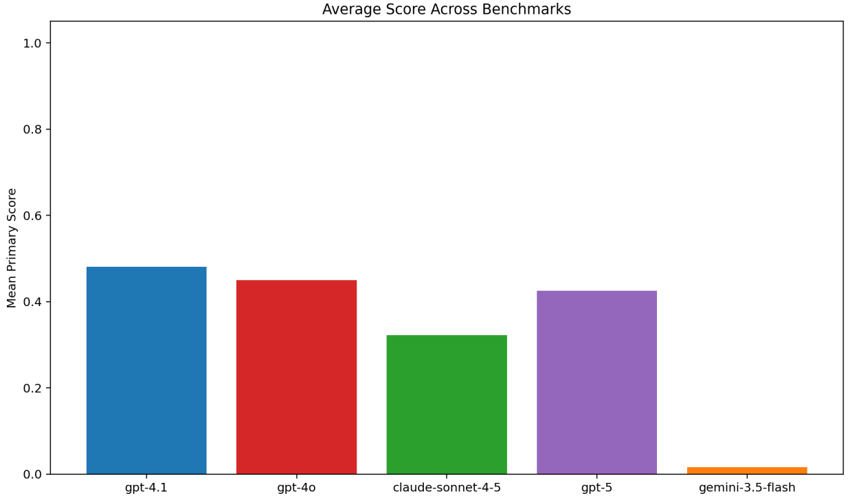
Figure 1: Mean score for the five API models on the shared June 10 overlap.
