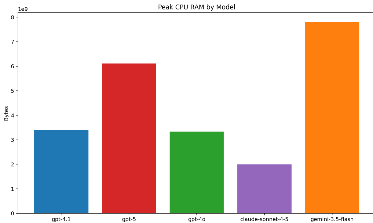
Figure 16: Peak CPU RAM by model.
