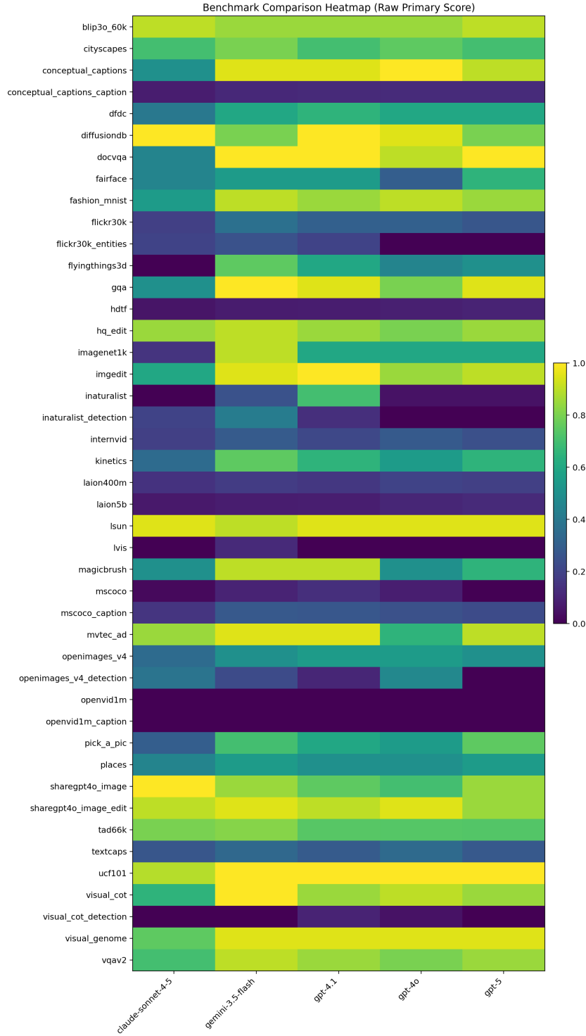
Figure 6: Raw primary score heatmap by benchmark and model.
