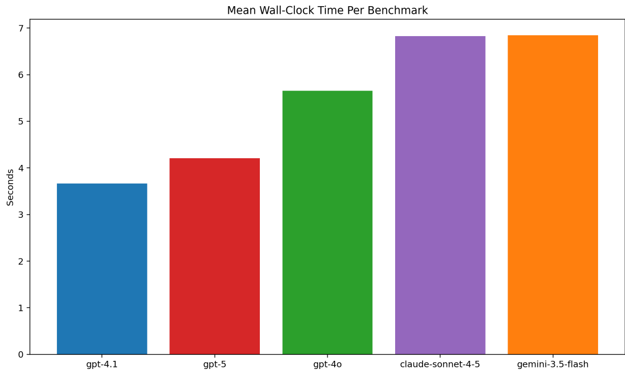
Figure 14: Mean wall-clock time per benchmark by model.
