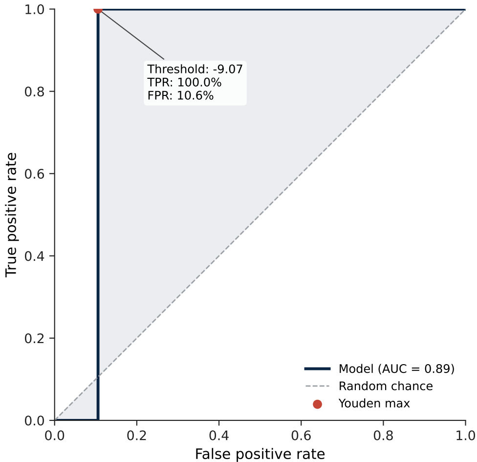
ROC Curve — Serotype 10C
