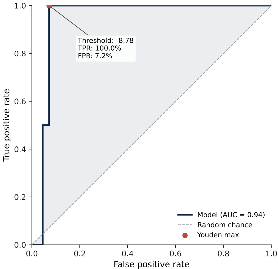
ROC Curve — Serotype 10X
