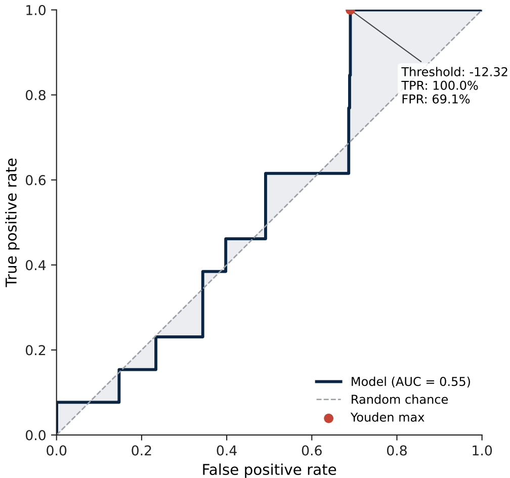
ROC Curve — Serotype 12B
