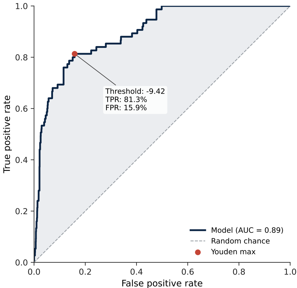
ROC Curve — Serotype 14
