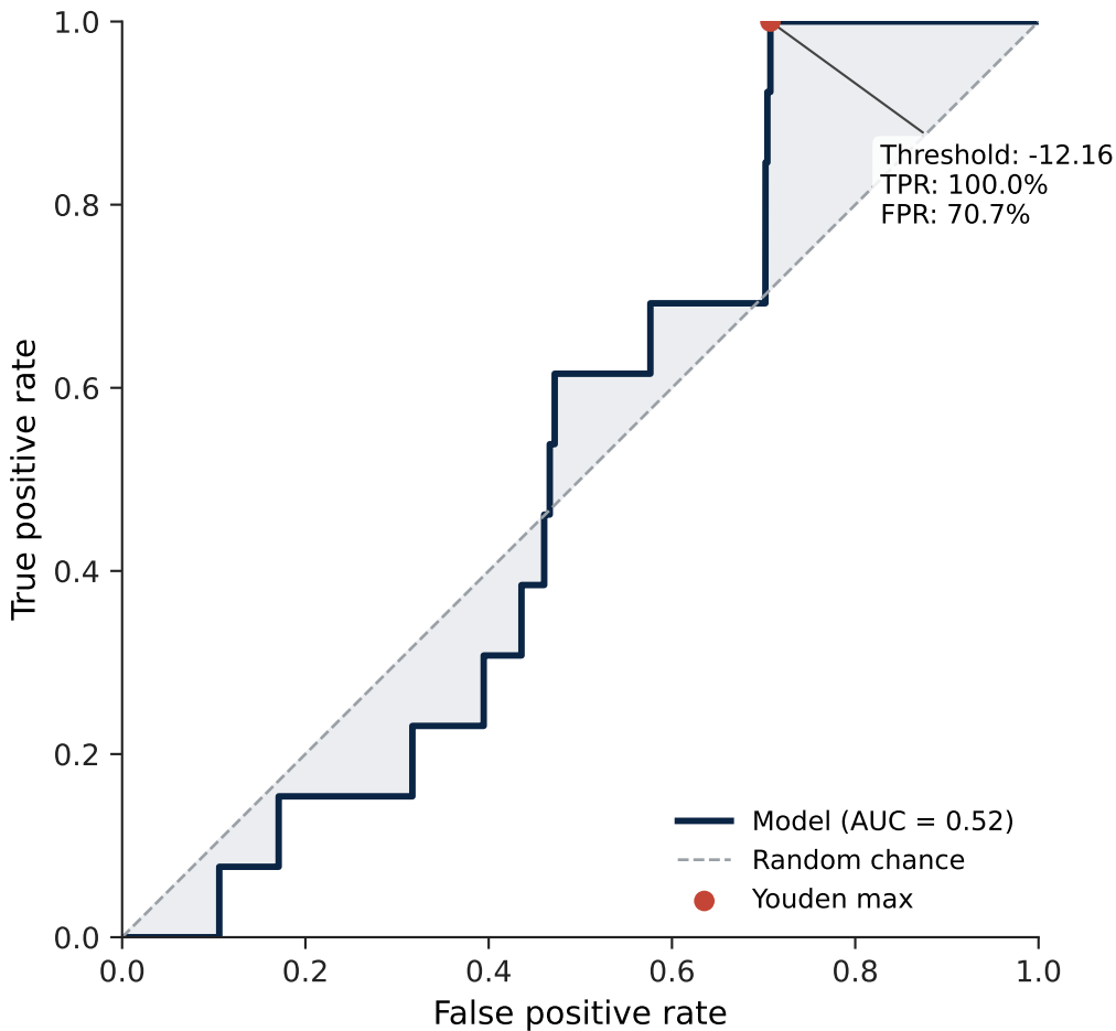
ROC Curve — Serotype 18B
