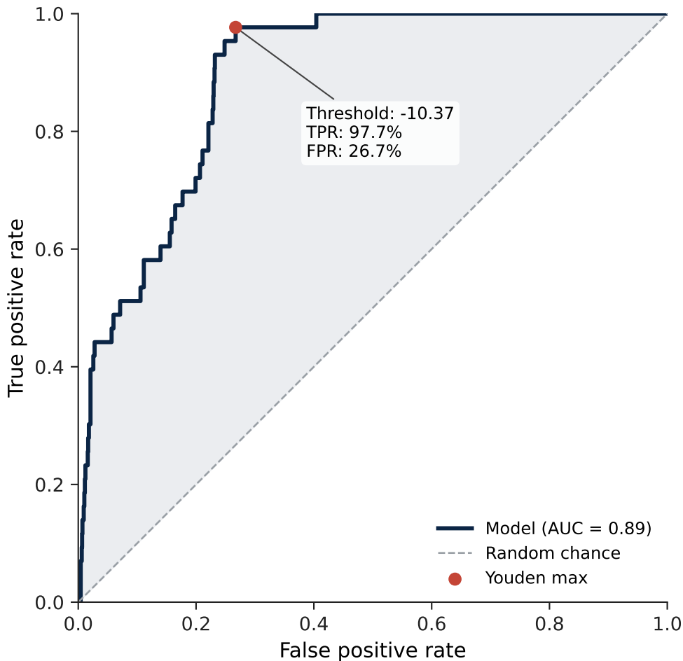
ROC Curve — Serotype 18C
