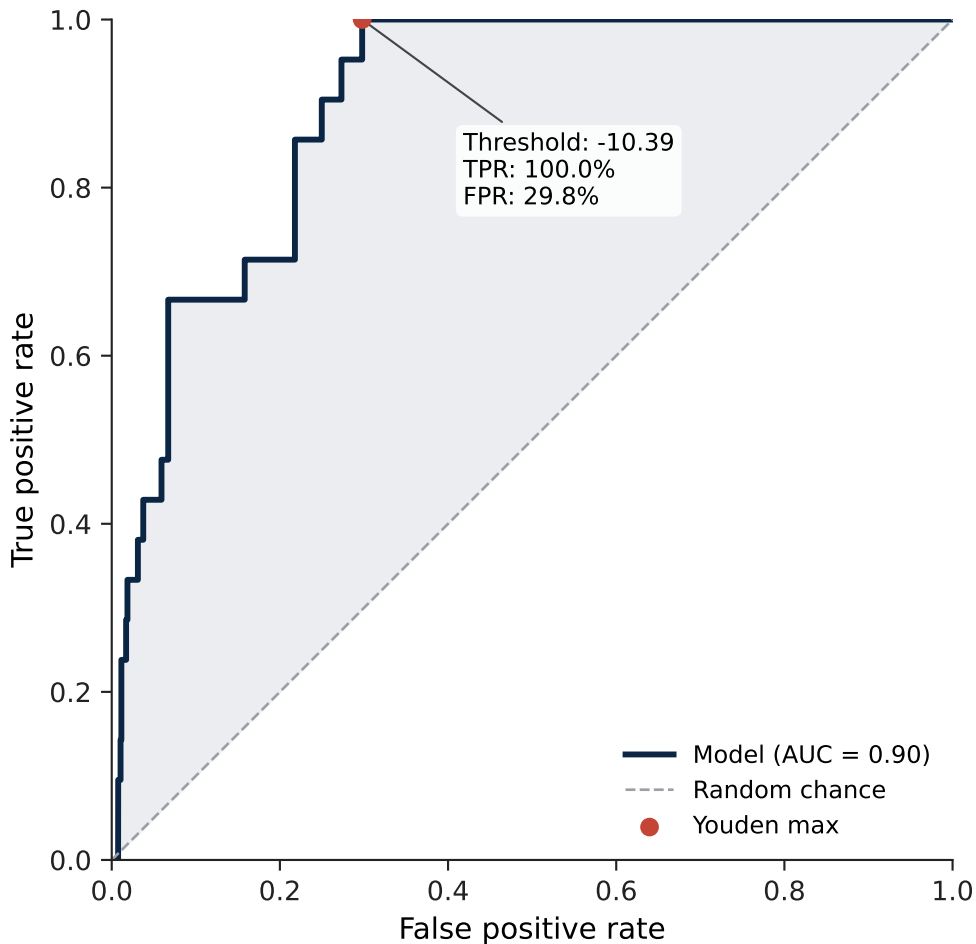
ROC Curve — Serotype 19B
