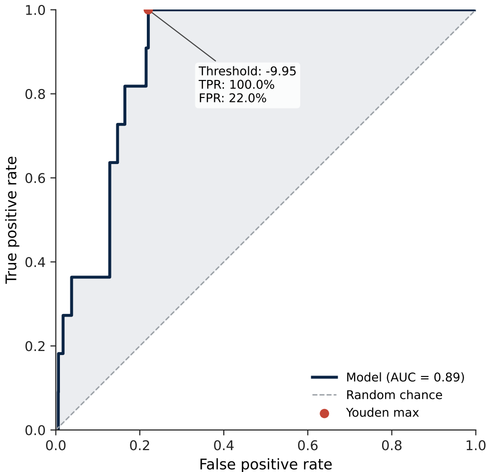
ROC Curve — Serotype 2
