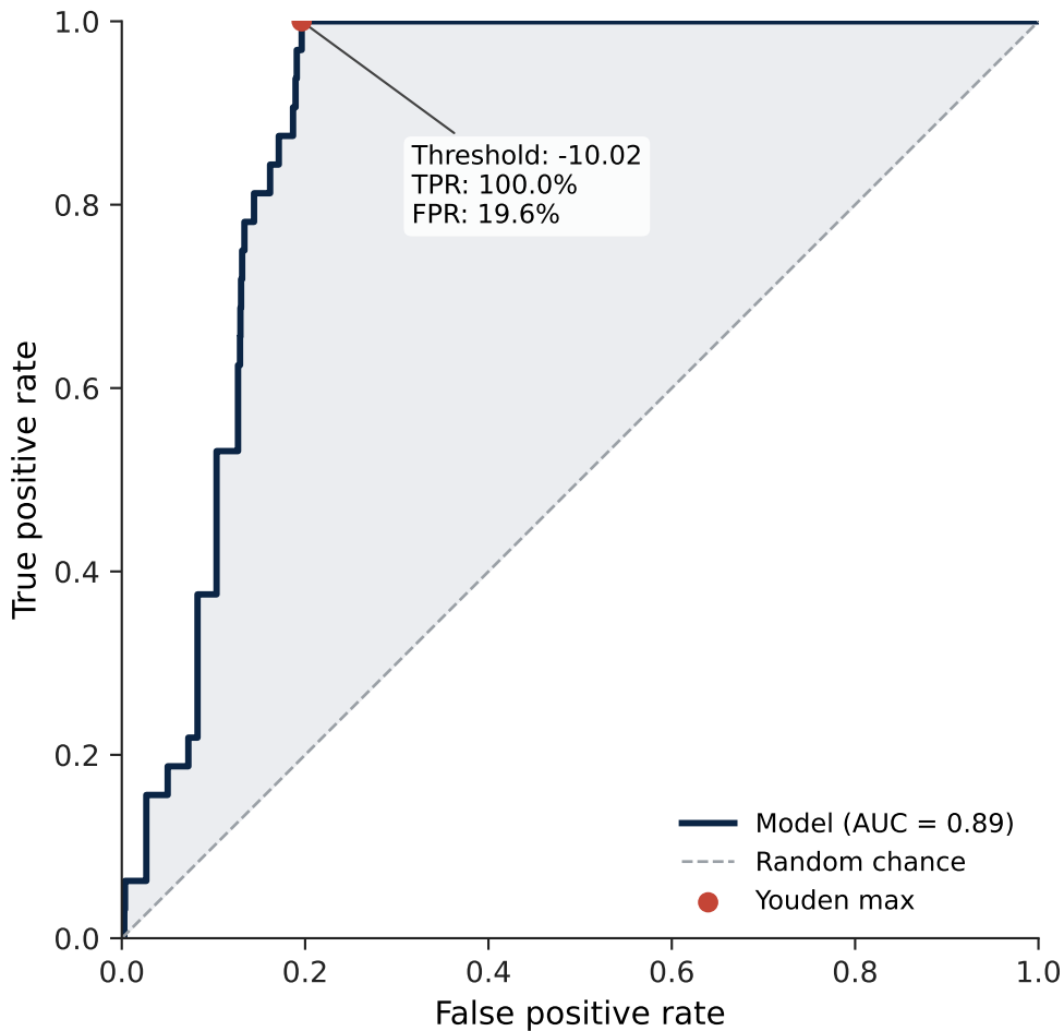
ROC Curve — Serotype 20B
