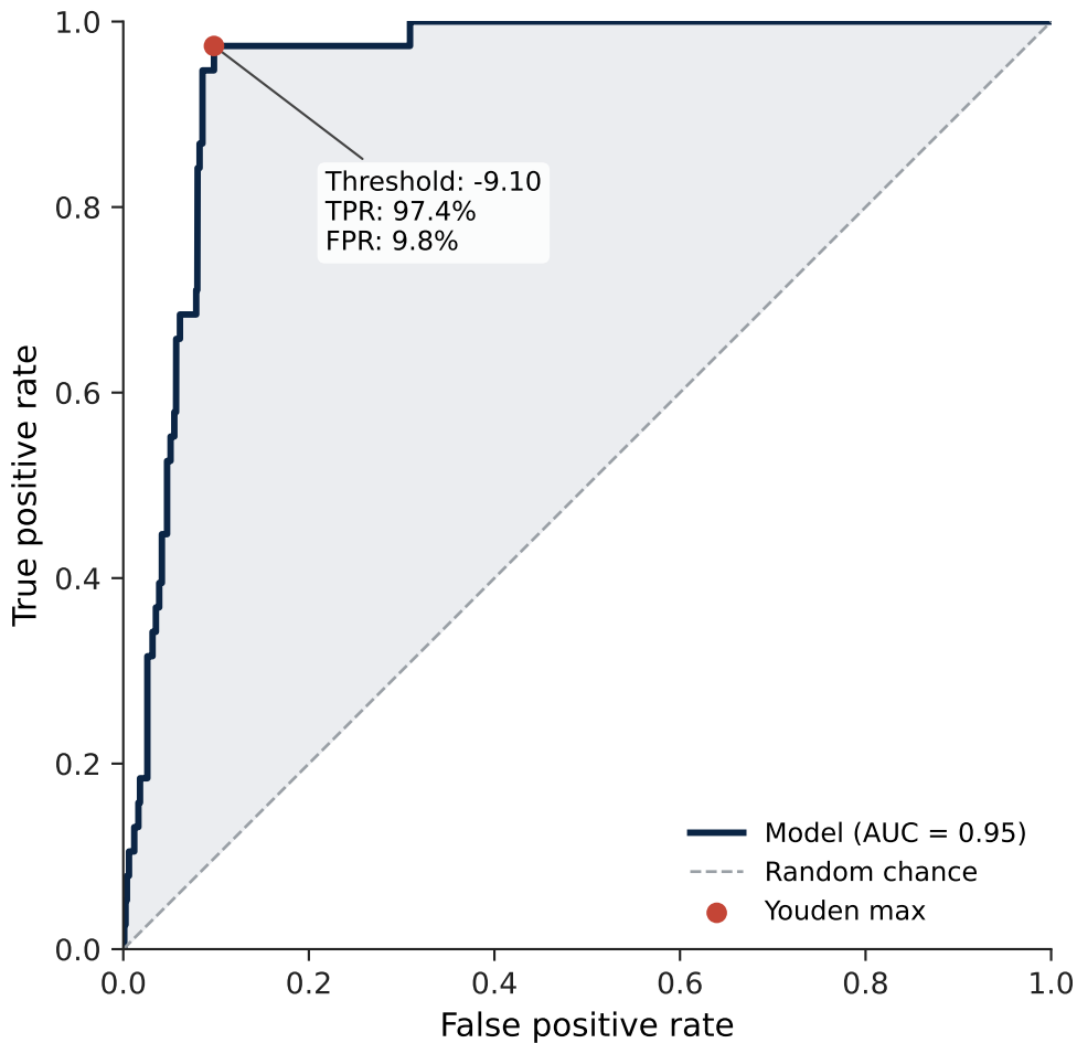
ROC Curve — Serotype 21
