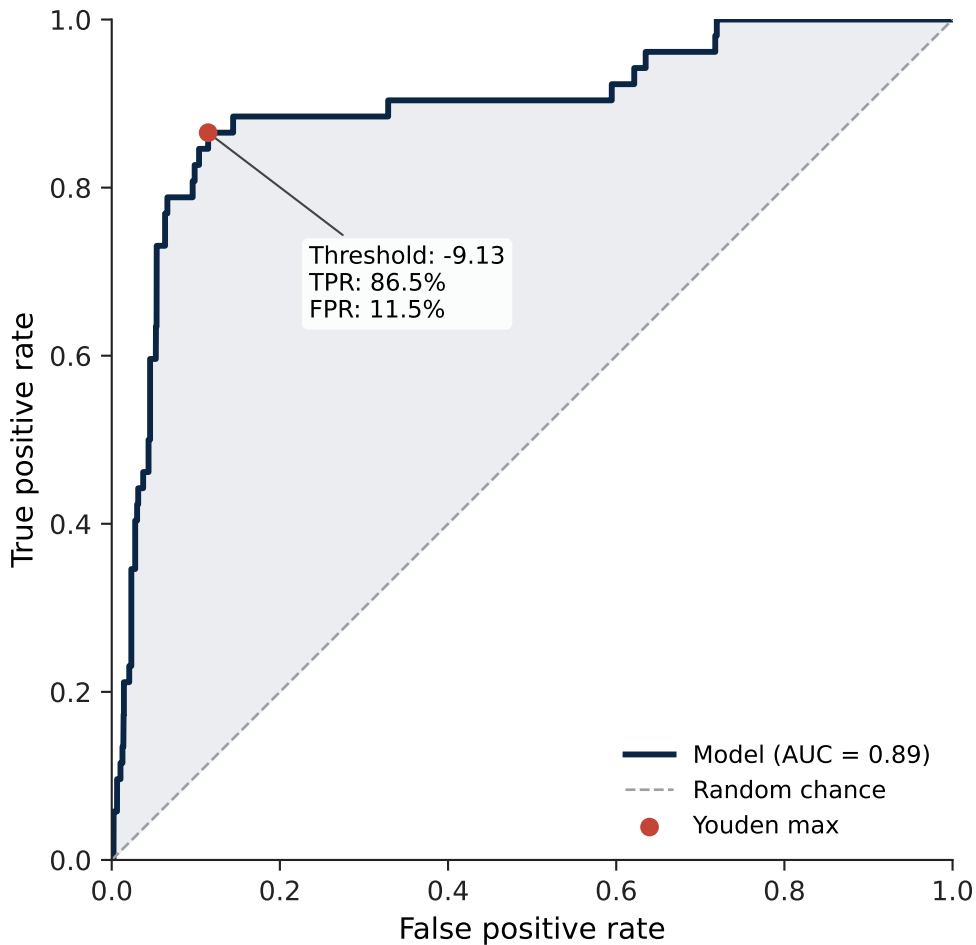
ROC Curve — Serotype 23B
