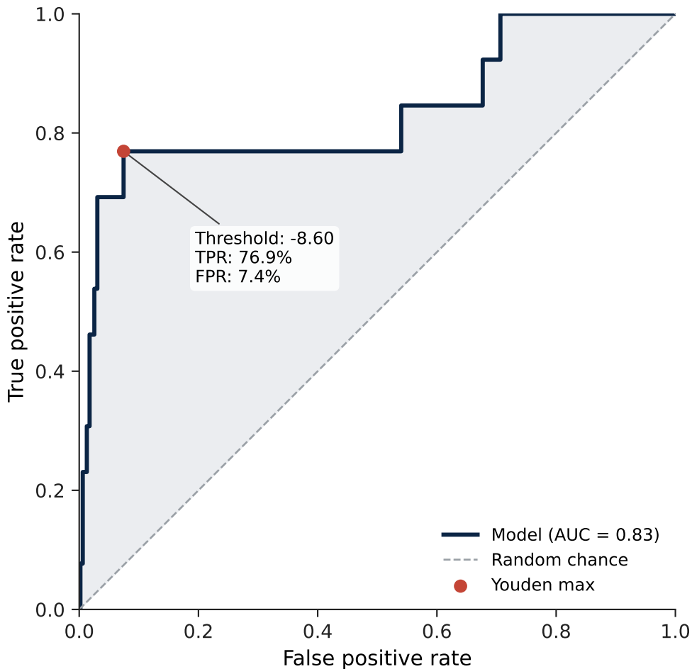
ROC Curve — Serotype 24A
