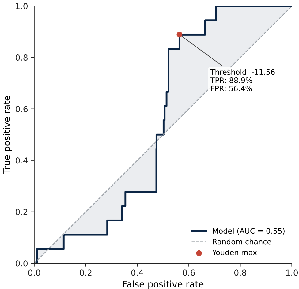
ROC Curve — Serotype 25F
