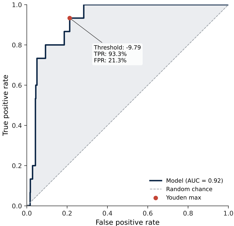
ROC Curve — Serotype 28A
