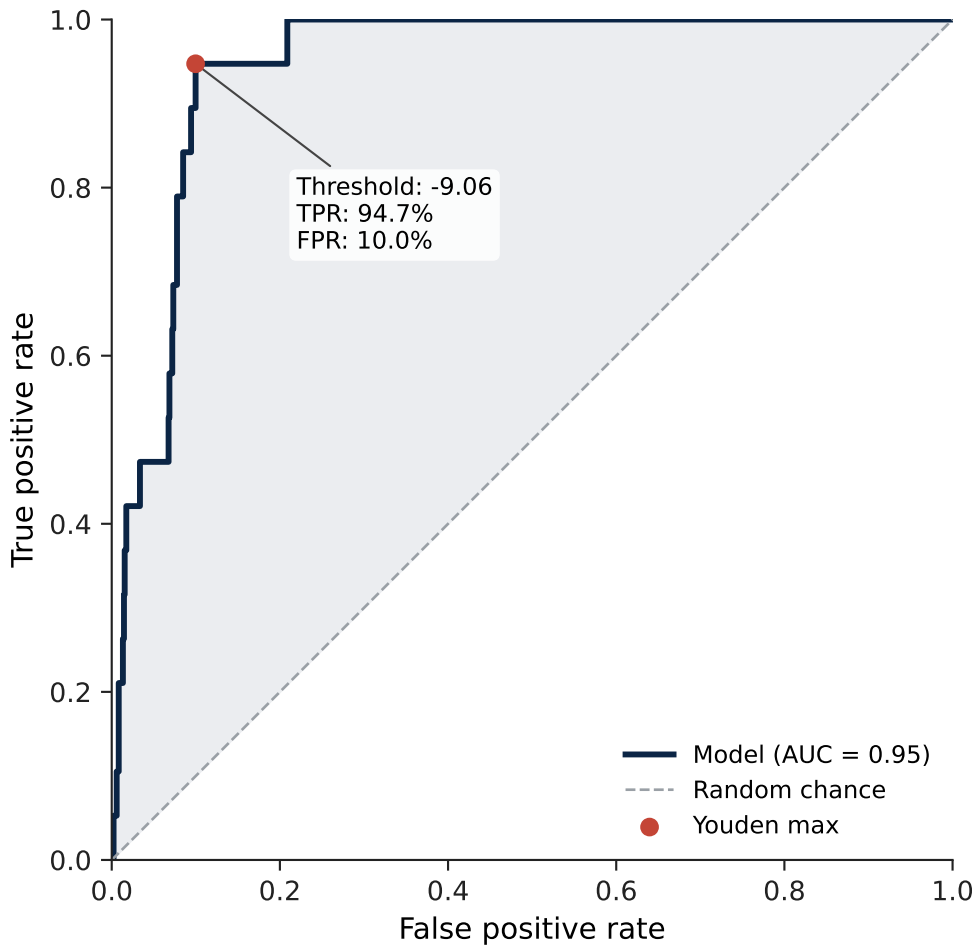
ROC Curve — Serotype 29
