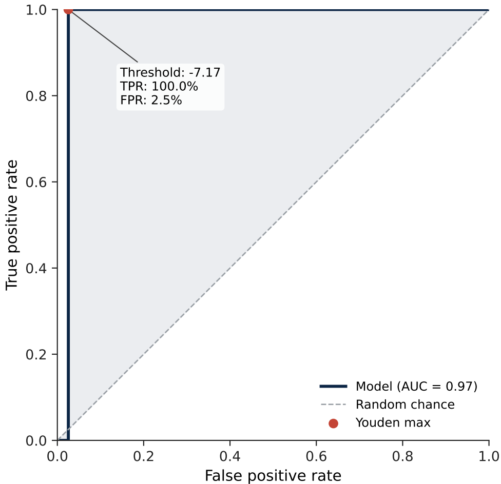
ROC Curve — Serotype 32
