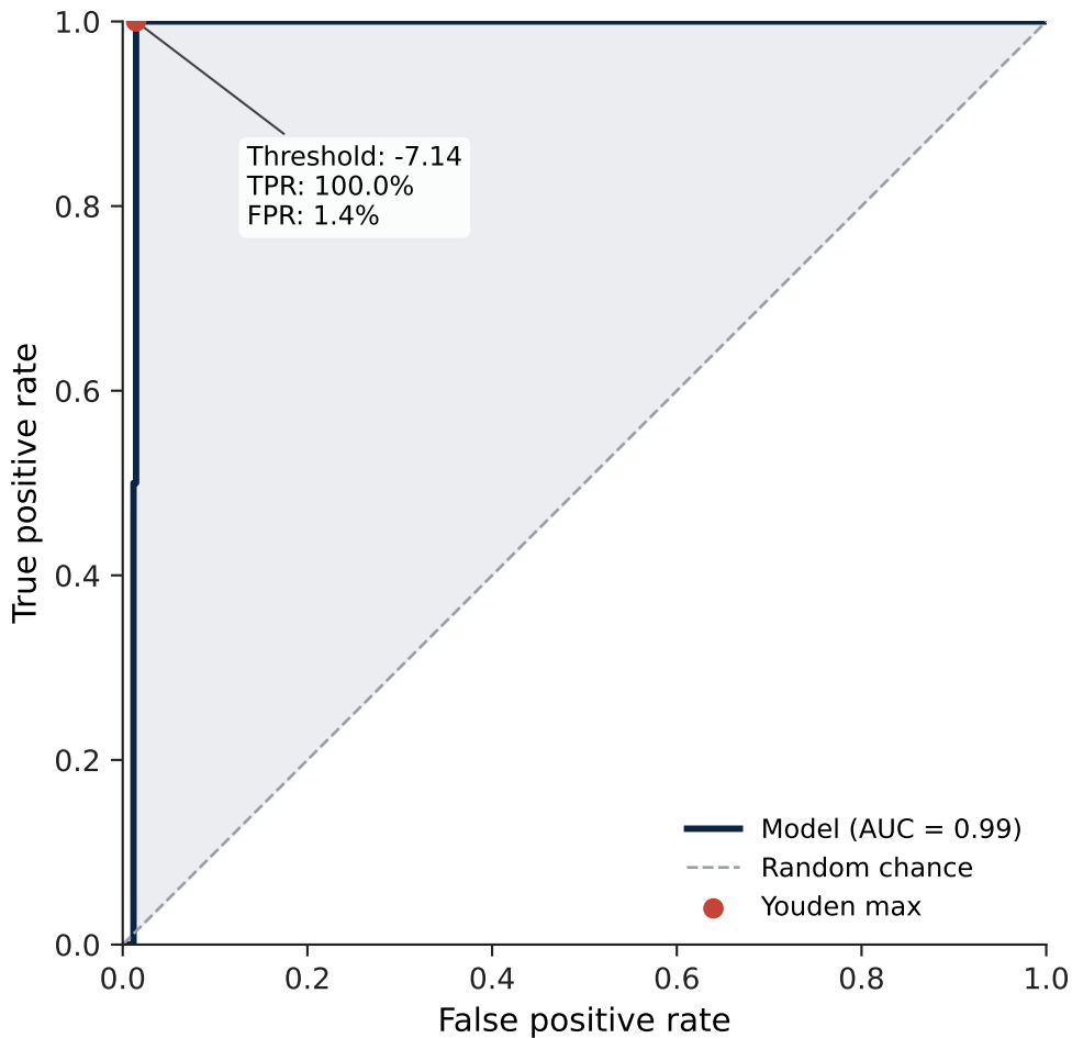
ROC Curve — Serotype 32F
