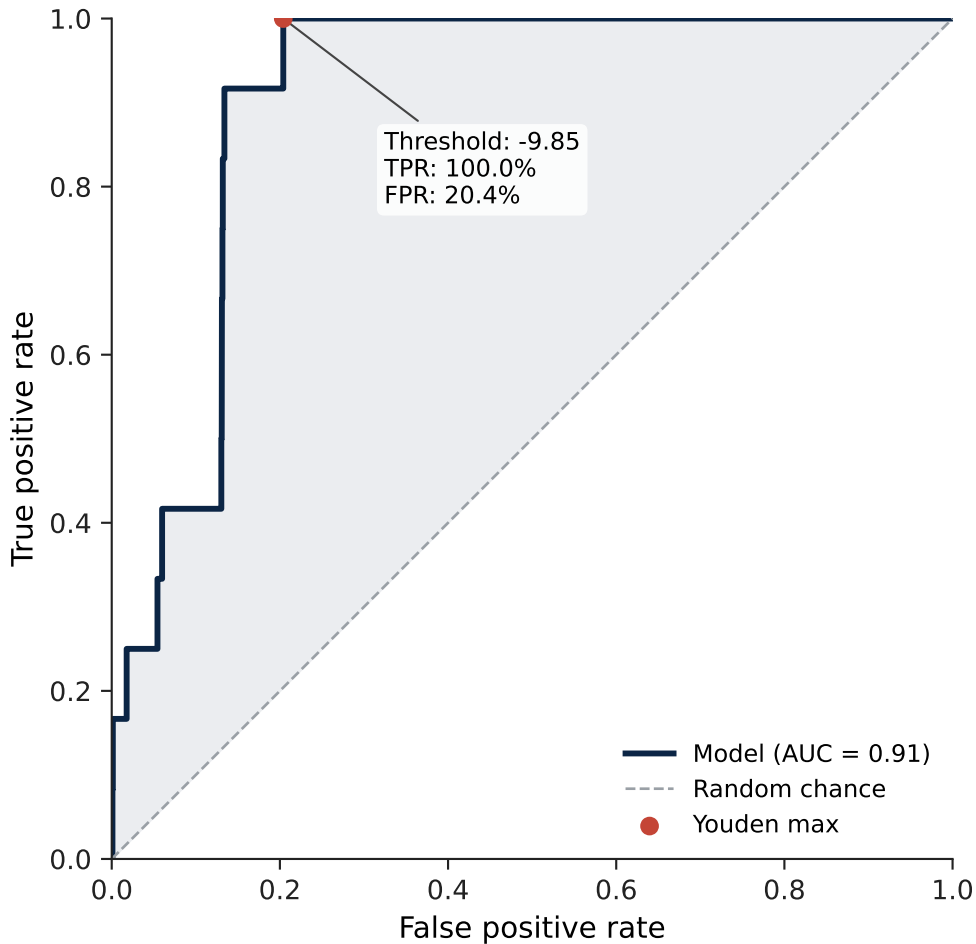
ROC Curve — Serotype 35A
