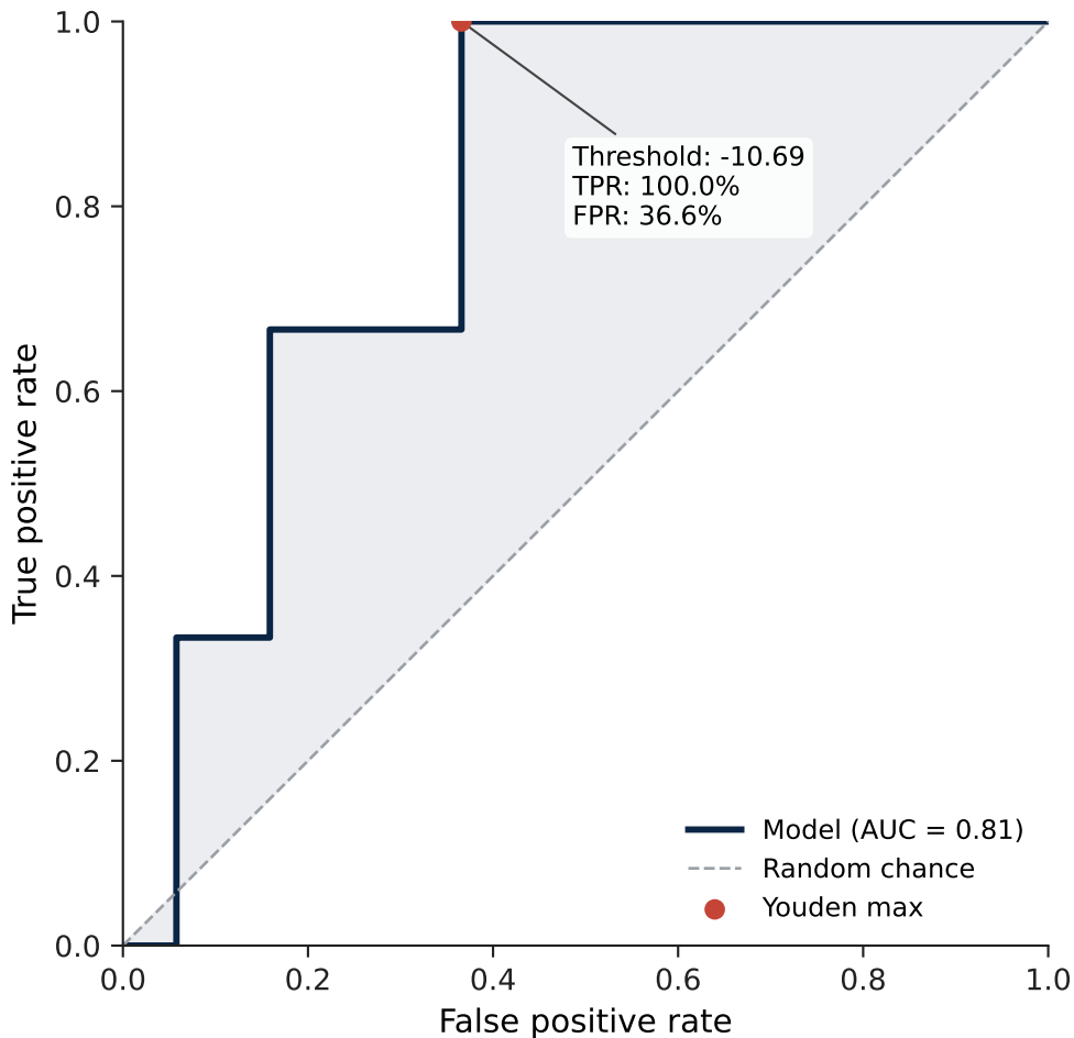
ROC Curve — Serotype 35B-35D
