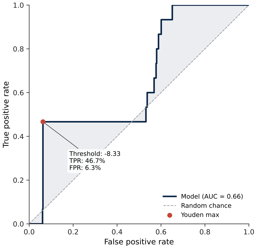
ROC Curve — Serotype 37
