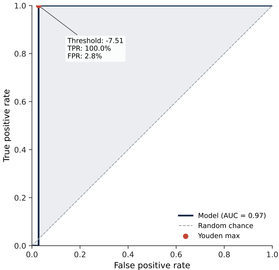
ROC Curve — Serotype 39X
