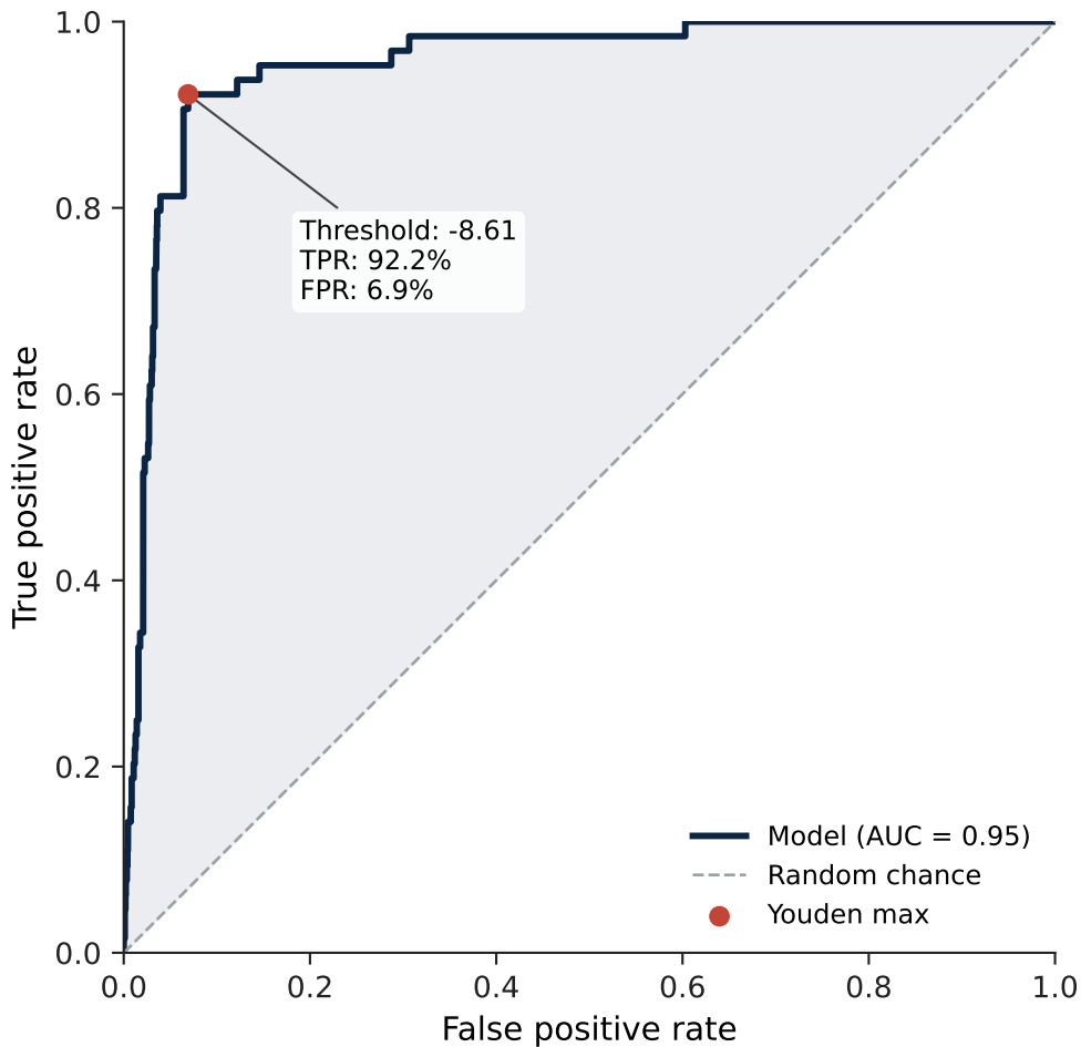
ROC Curve — Serotype 4
