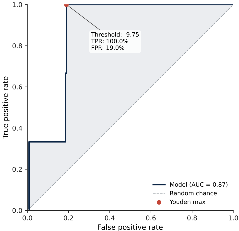
ROC Curve — Serotype 42
