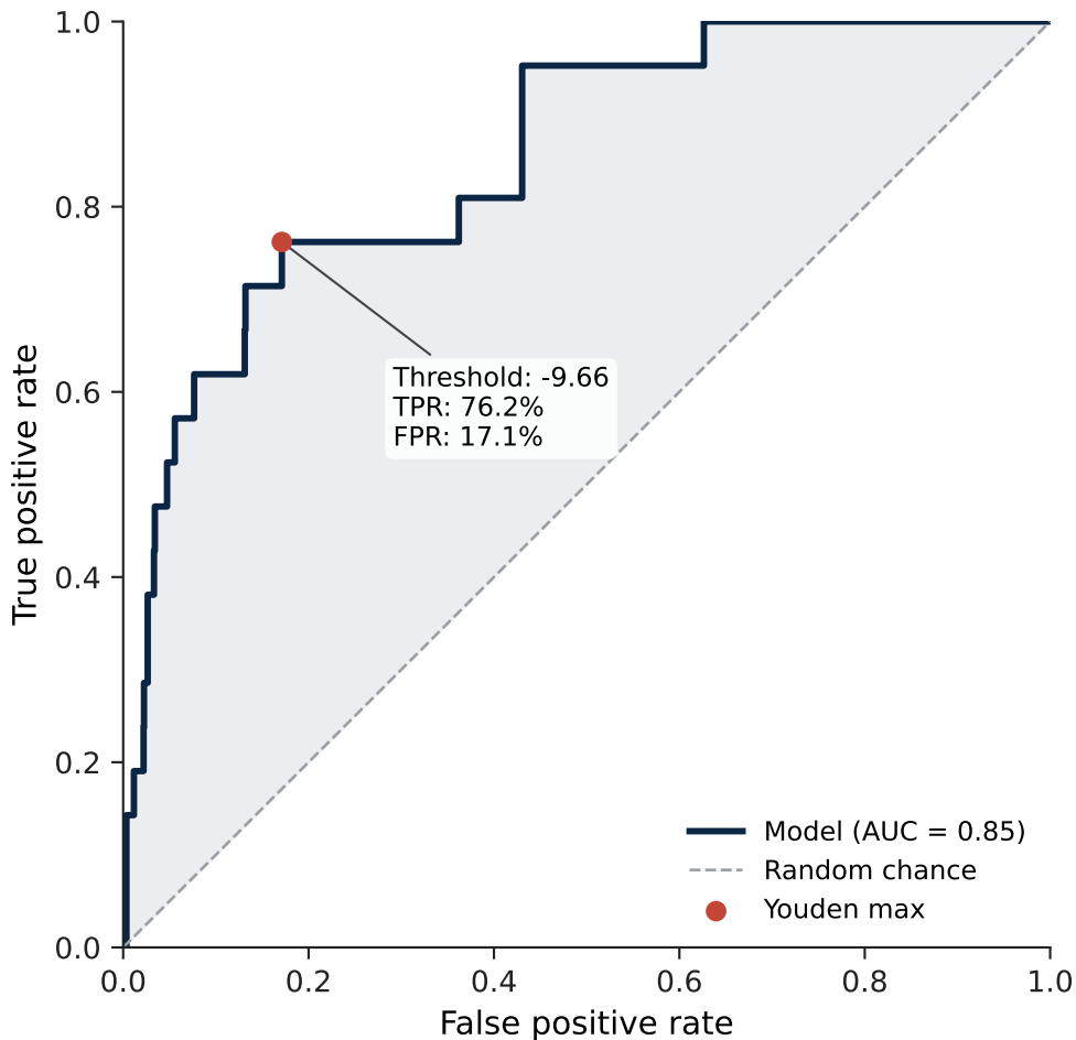
ROC Curve — Serotype 46
