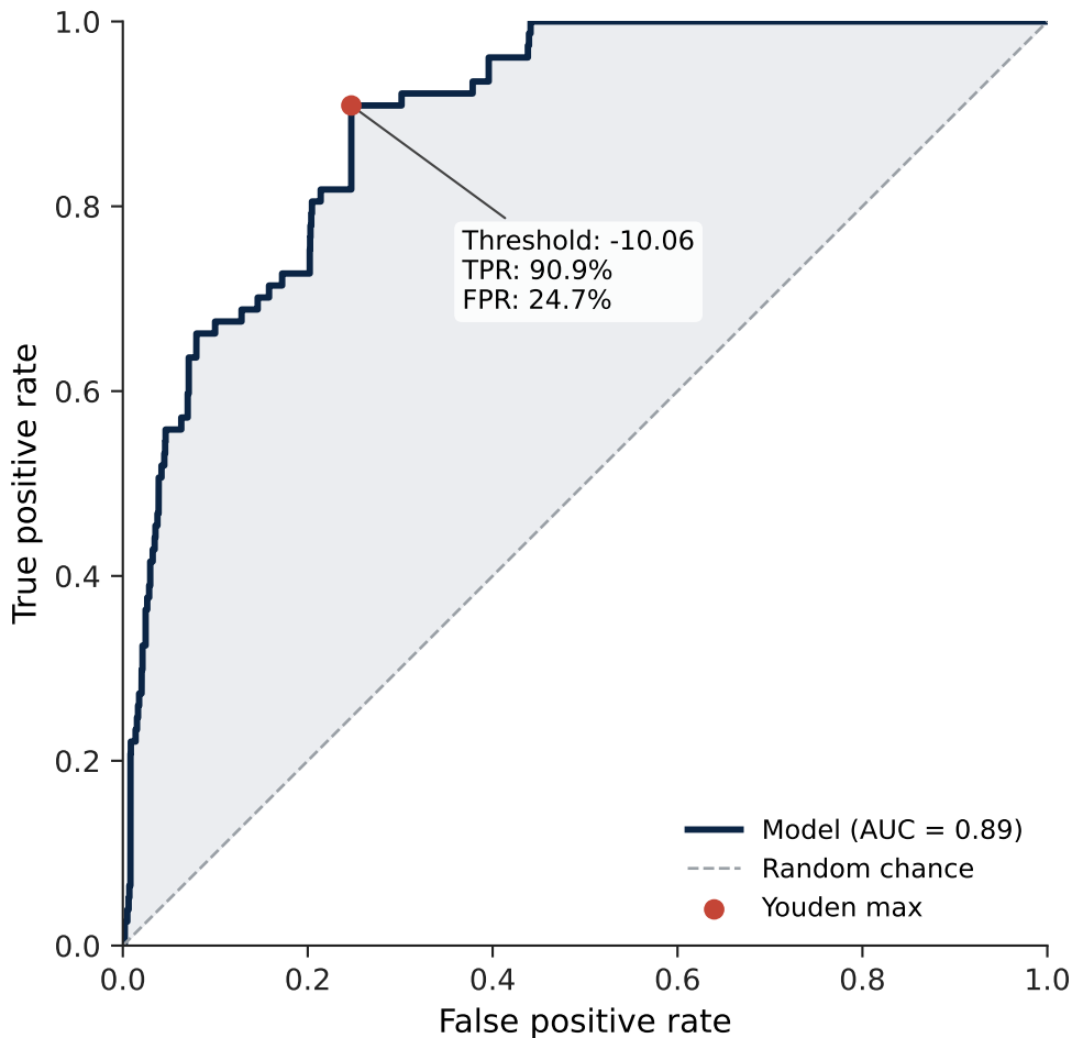
ROC Curve — Serotype 6A
