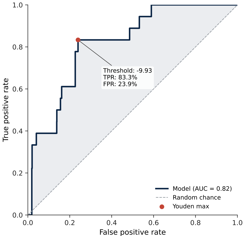
ROC Curve — Serotype 6D
