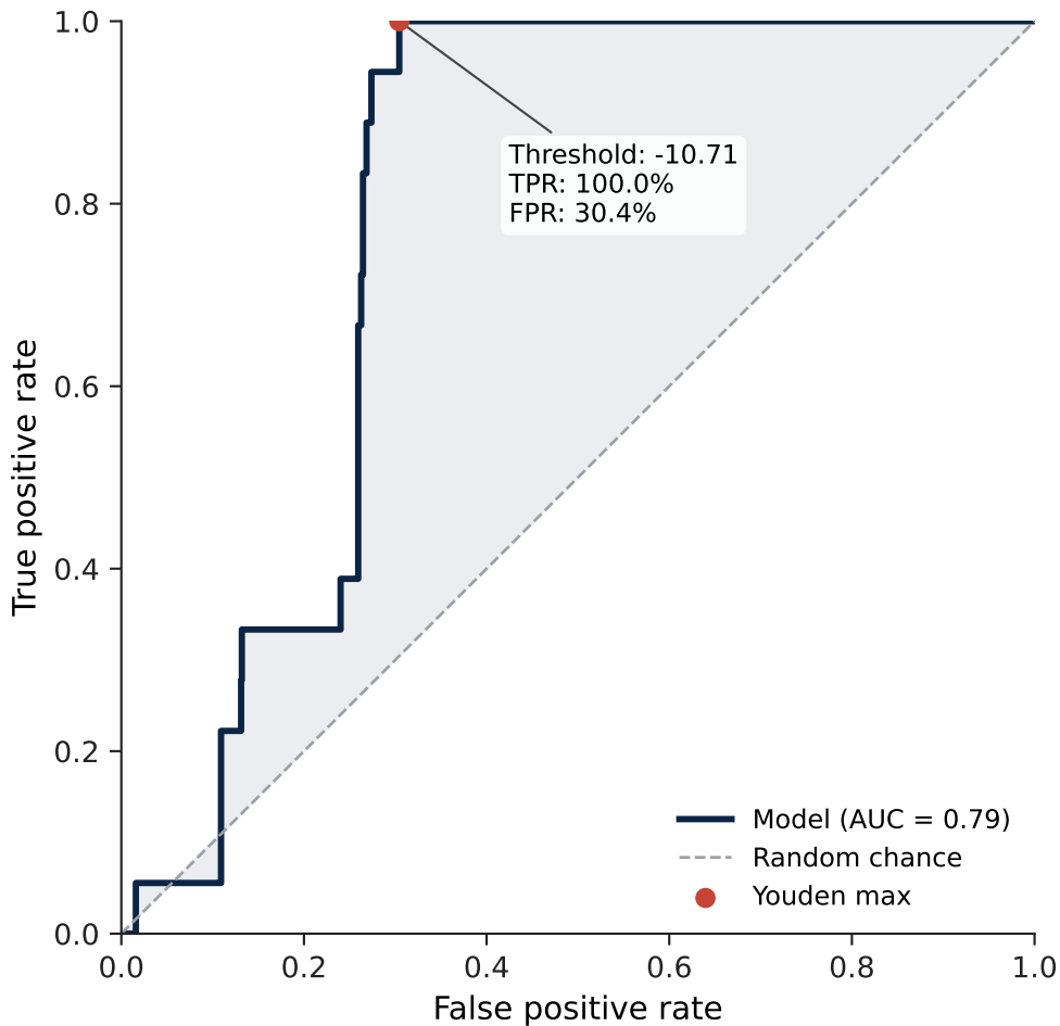
ROC Curve — Serotype 6E
