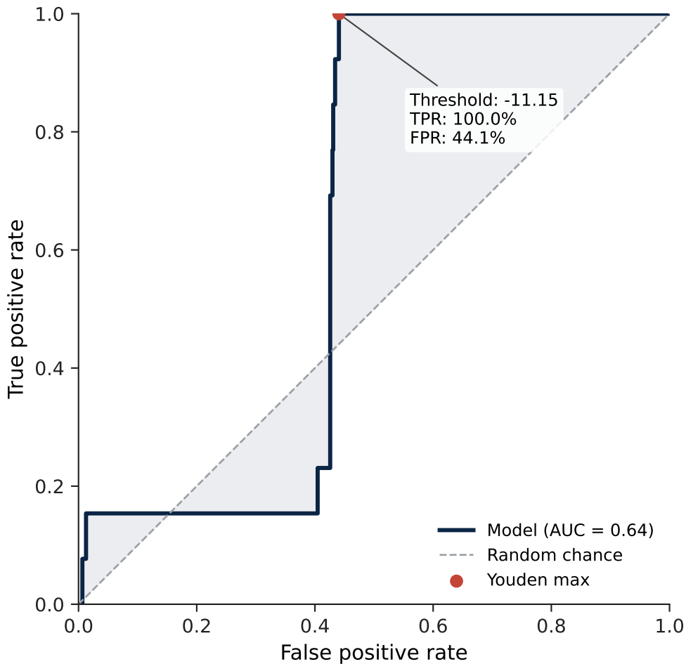
ROC Curve — Serotype 7B
