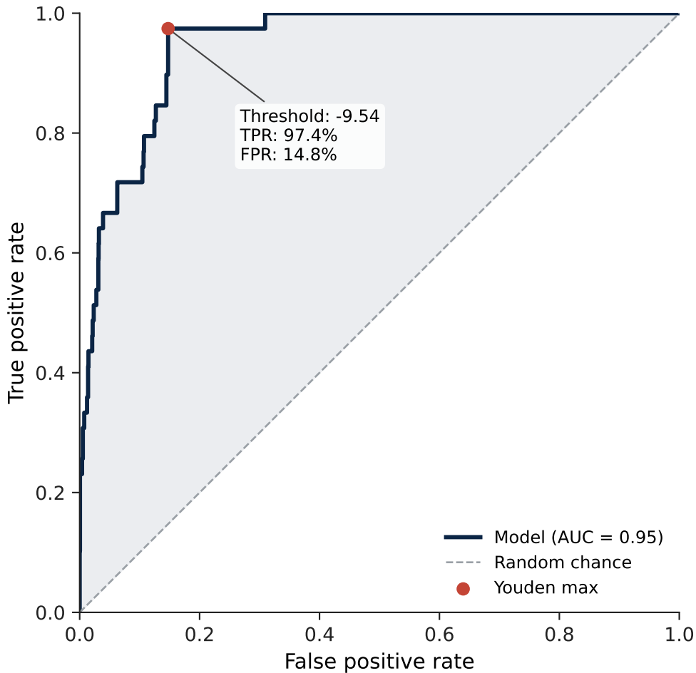
ROC Curve — Serotype 7C
