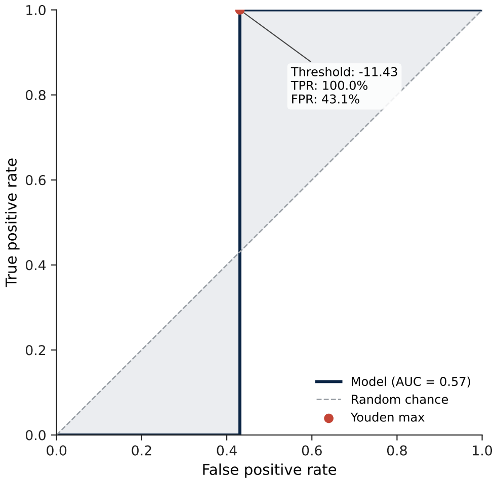
ROC Curve — Serotype 9A
