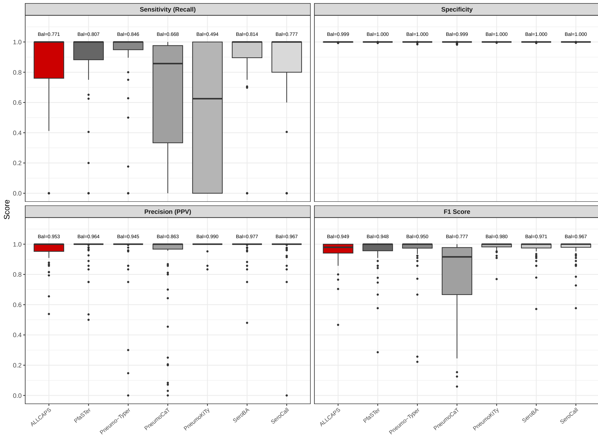
UK_benchmark – serotype_exact
